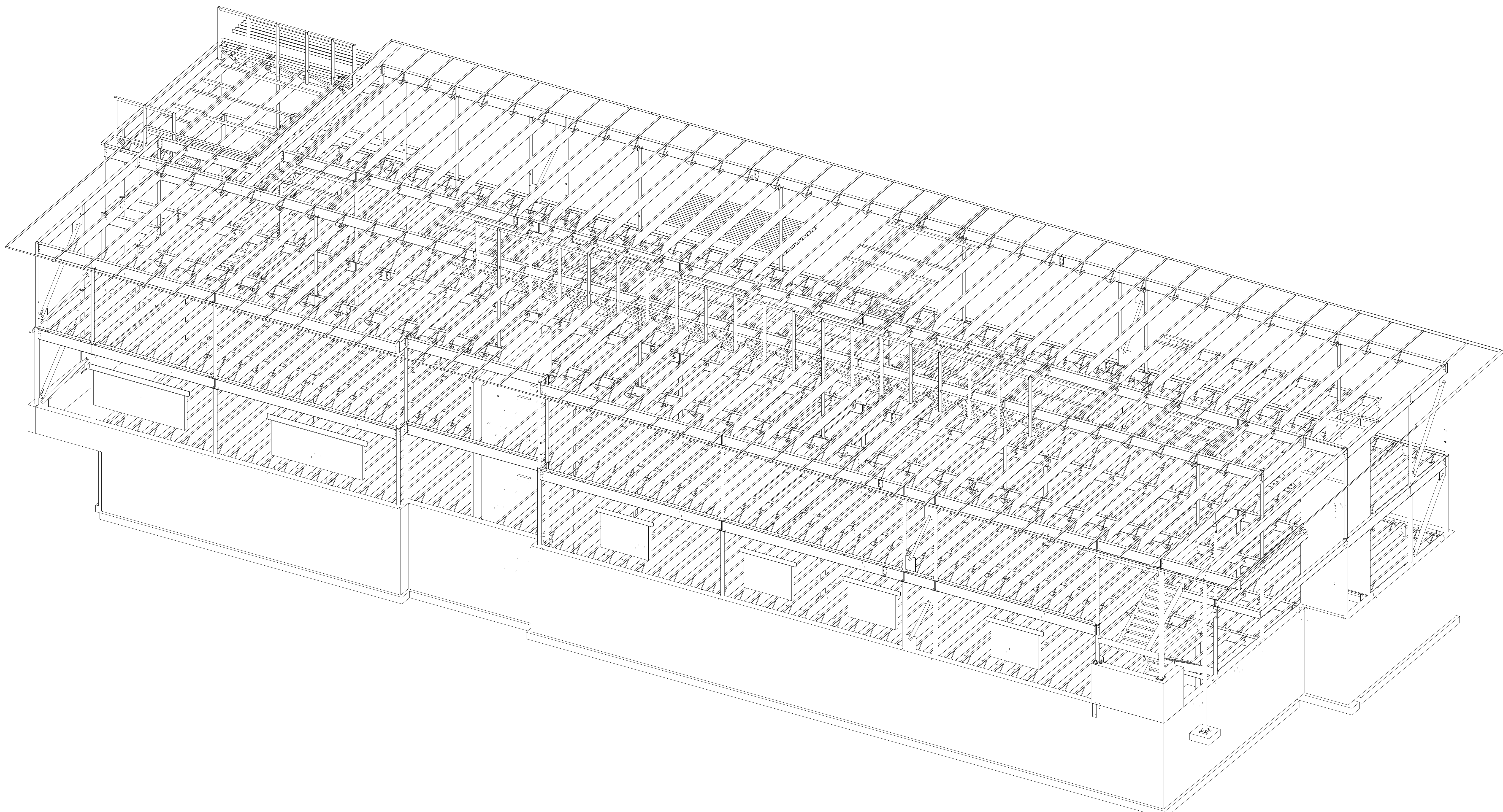
ISOMETRIC VIEW
